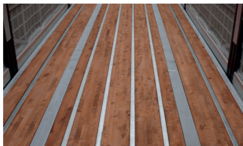
Glue-laminated solid hardwood with steel omega profiles
