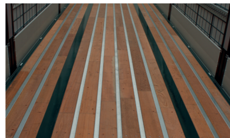
Anti-puncture solid hardwood with steel omega profiles
