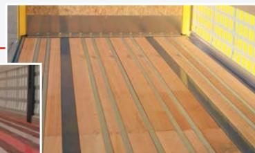
Solid hardwood planks Steel omega profiles resistant against punching
