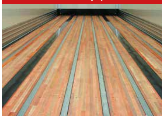
Laminated hardwood floor 35 mm thick with steel omega profiles
